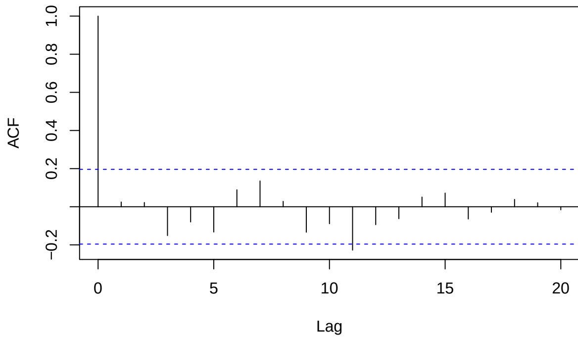
Series resid(mod11)
