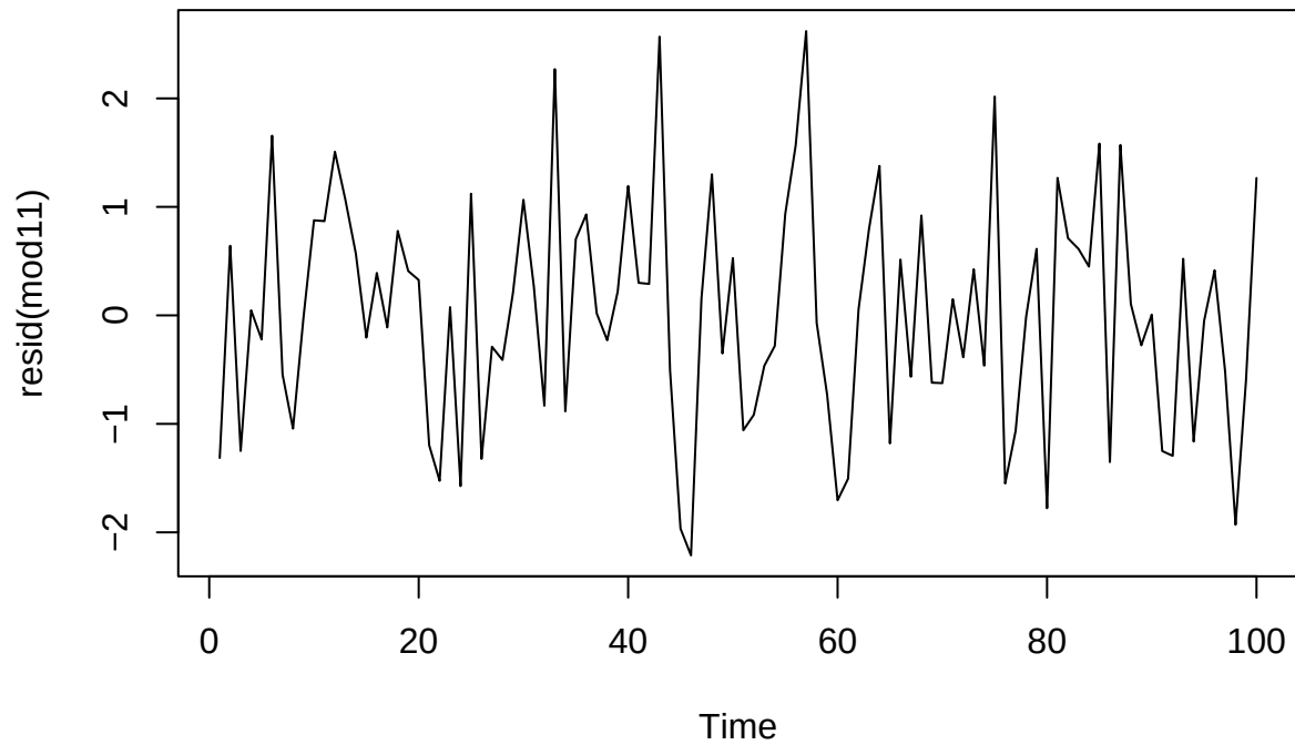
Series resid(mod11)
